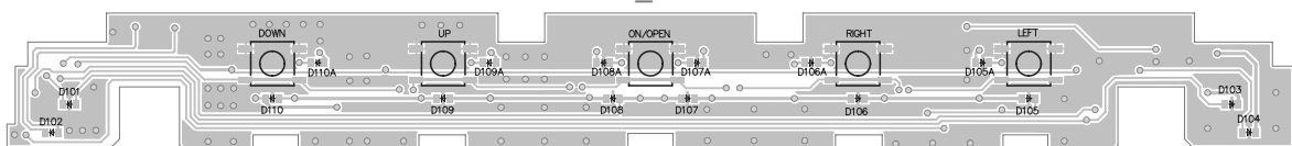
RFM769_305 PCB LAYOUT
