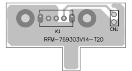
RFM769_303 PCB LAYOUT
