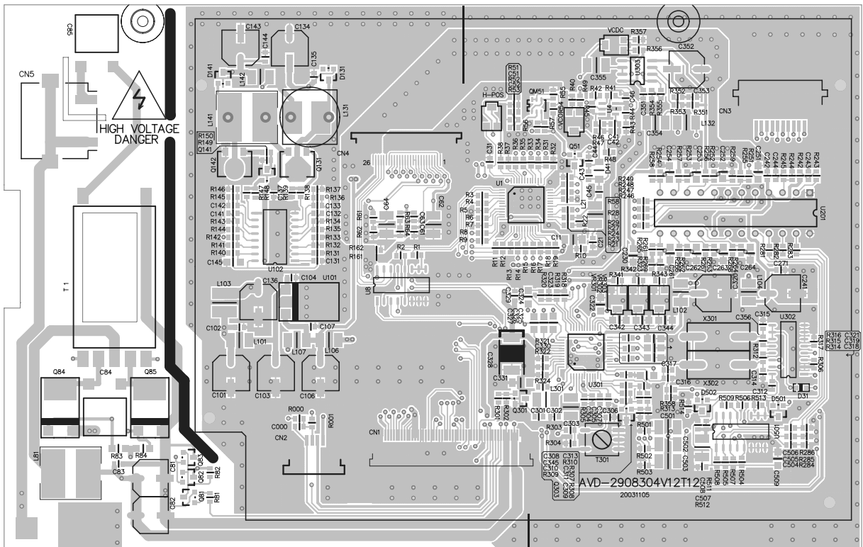
RFM769_305 PCB LAYOUT
